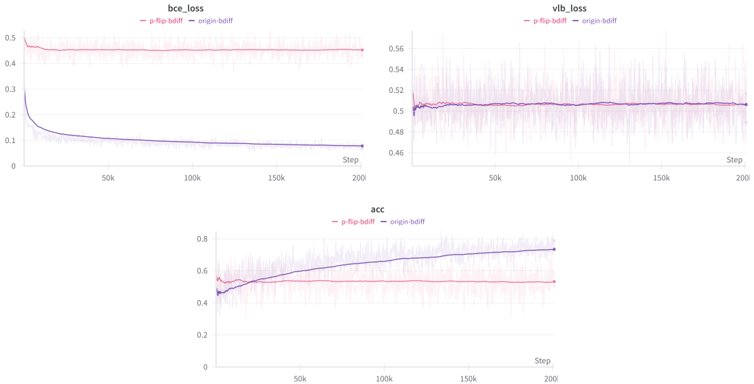
FIGURE 5.4: Comparison between models with different prediction target: flip probability and original pose .
